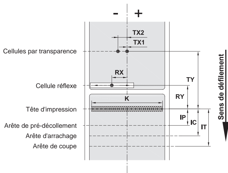
Figure 25 Dimensions
