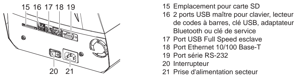
Figure 3 Connexions
