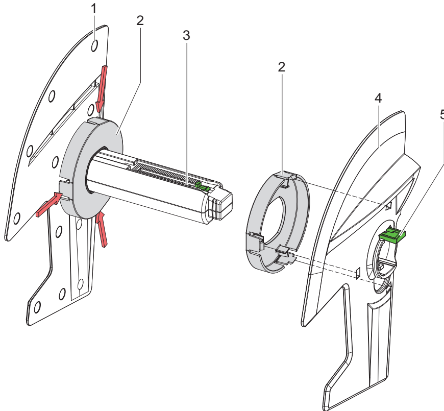
Figure 10 Adaptation du support de rouleau
